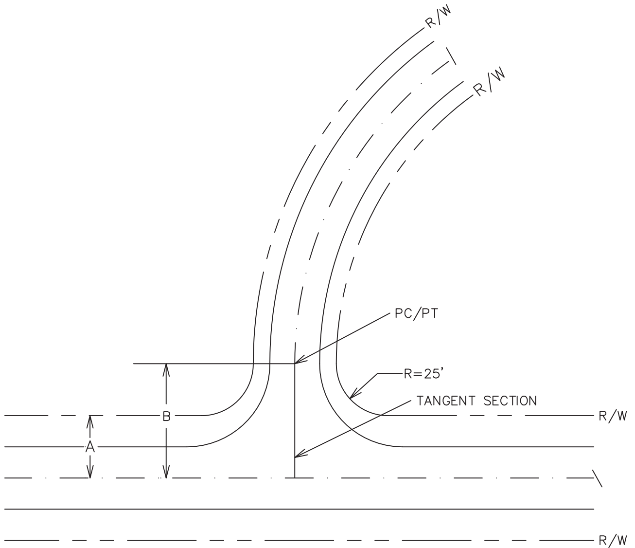
INTERSECTION DIAGRAM
