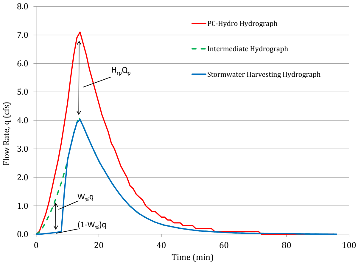
Figure G.2. Stormwater harvesting hydrograph with H_{rp} = 0.436 and W_A = 0.95 .
